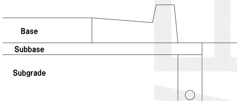
Figure D4.1 - Typical Subsoil Drain
