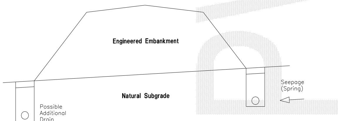
Figure D4.3 - Foundation Drains
