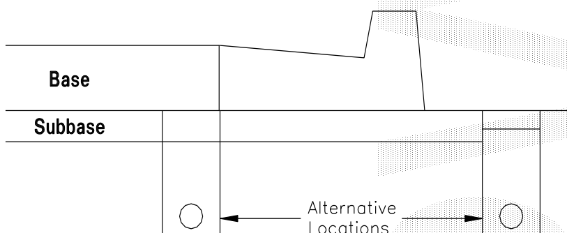
Figure D4.2 - Typical Subpavement Drain
