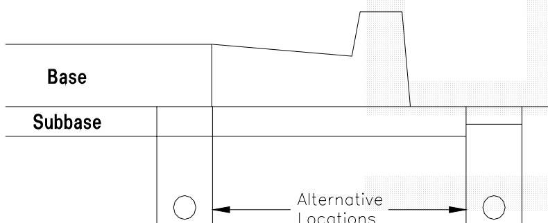
Figure D4.1 - Typical Subsoil Drain
