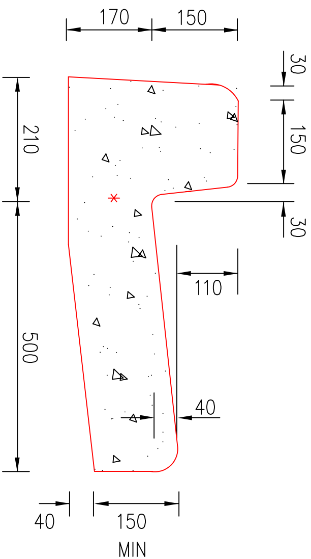
STANDARD KERB & GUTTER (SA)
