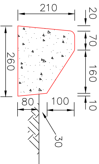
MOUNTABLE KERB (SF)
