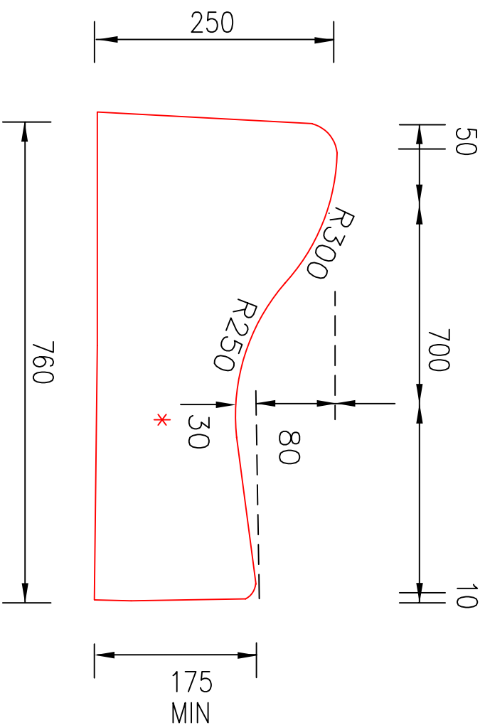
ROLL KERB & GUTTER (RT)
