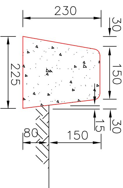
KERB ONLY OR BARRIER KERB (SM)
