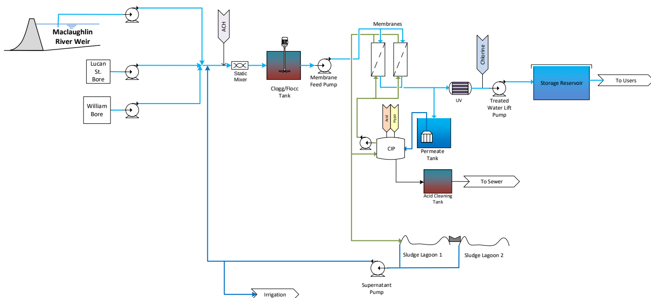
Figure 6-13: Schematic of the Nimmitabel Membrane Filtration WTP.
