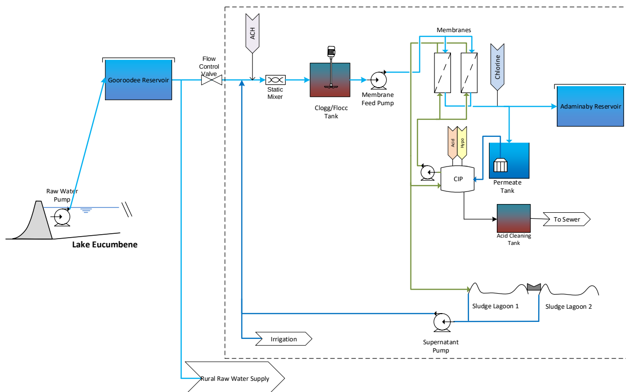
Figure 5-10: Schematic of the Adaminaby Membrane Filtration WTP.
