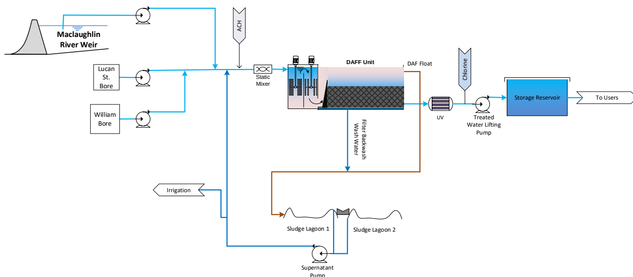
Figure 6-14: Schematic of the Nimmitabel DAFF WTP.
